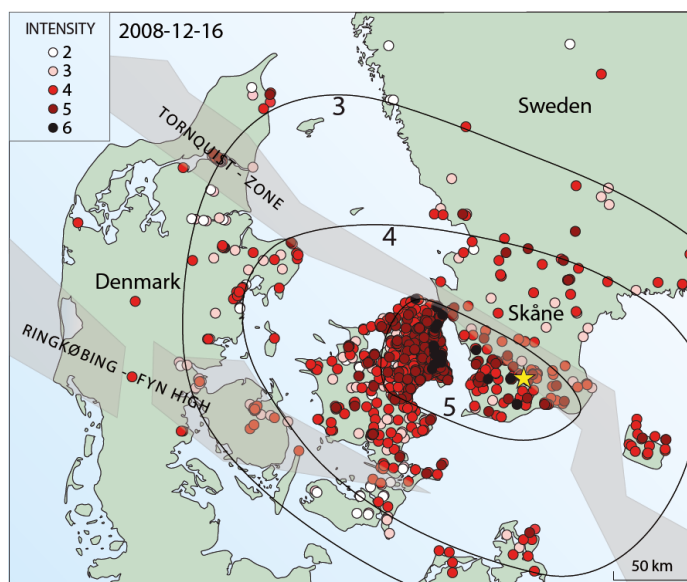
Figure 44. The earthquake in Scania (Skåne) in 2008 was registered in many areas in eastern Denmark as shown on the Intensity map from Voss et al., (2009).
