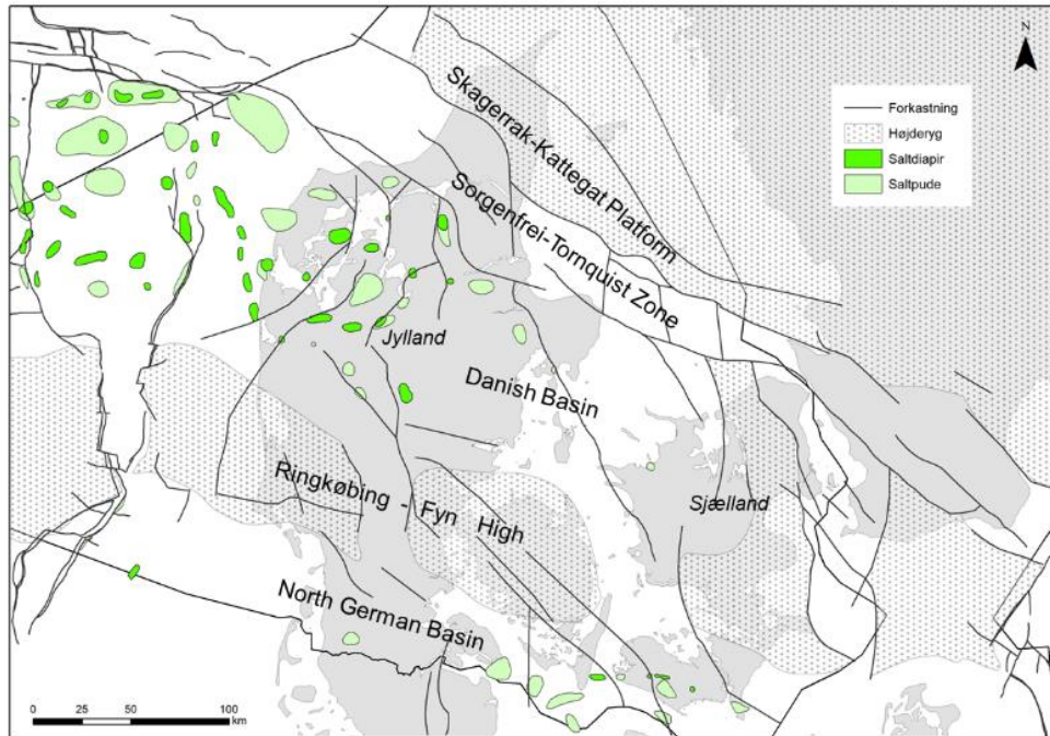
Figure 10. Map showing the occurrence of Zechstein salt pillows and diapirs.
