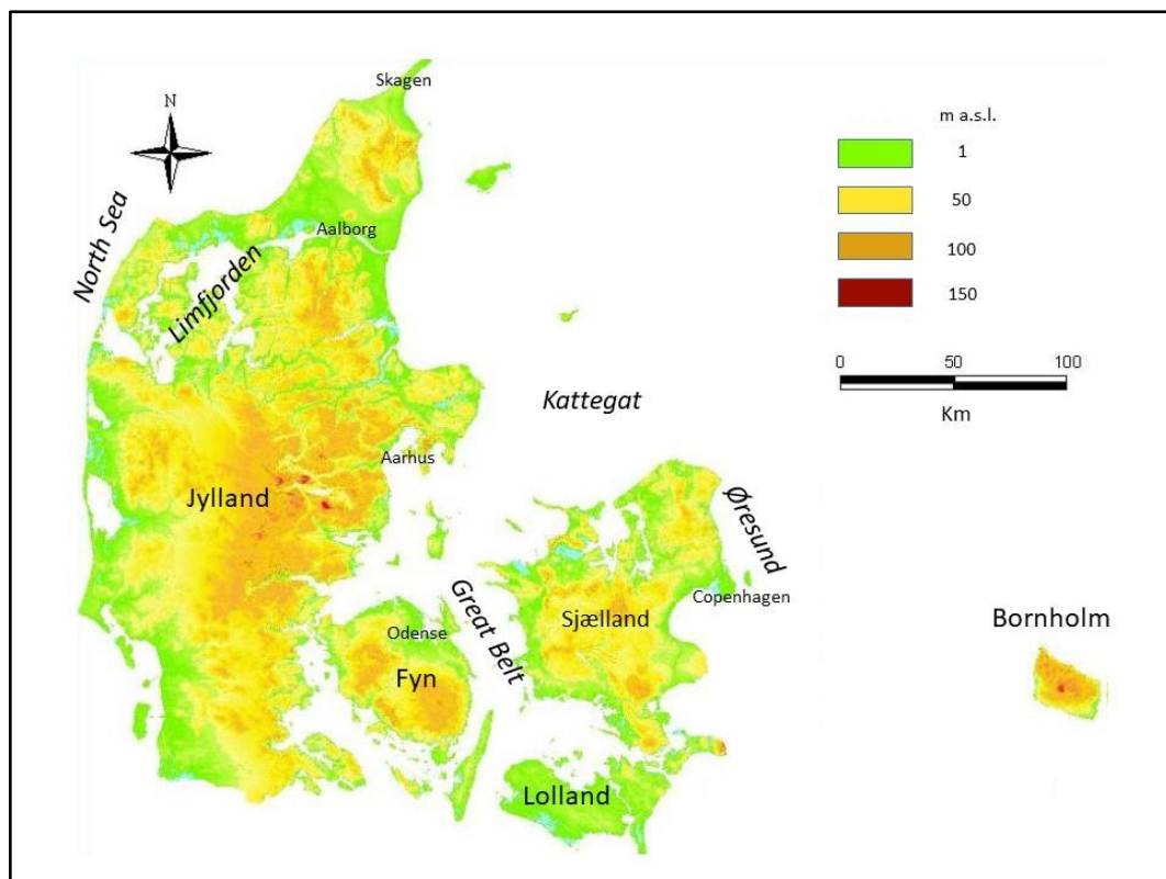
Figure 1. Topographic map of Denmark showing the general low relief landscape with the highest elevations being less than 200 meters above mean sea level. The highest areas are found in the central part of Sjælland, the central part of Fyn, the central part of Bornholm and the central part of Jylland.
