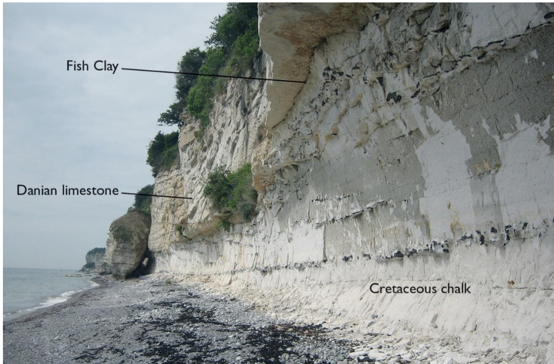
Figure 19. Danian limestone overlying the Cretaceous chalk at the Stevns Cliff. Both types of limestone contain layers of black and grey chert. The boundary between the Cretaceous succession and the Tertiary (C-T boundary) is represented by the presence of the black Fish Clay layer (as marked at the base of the overhang).
