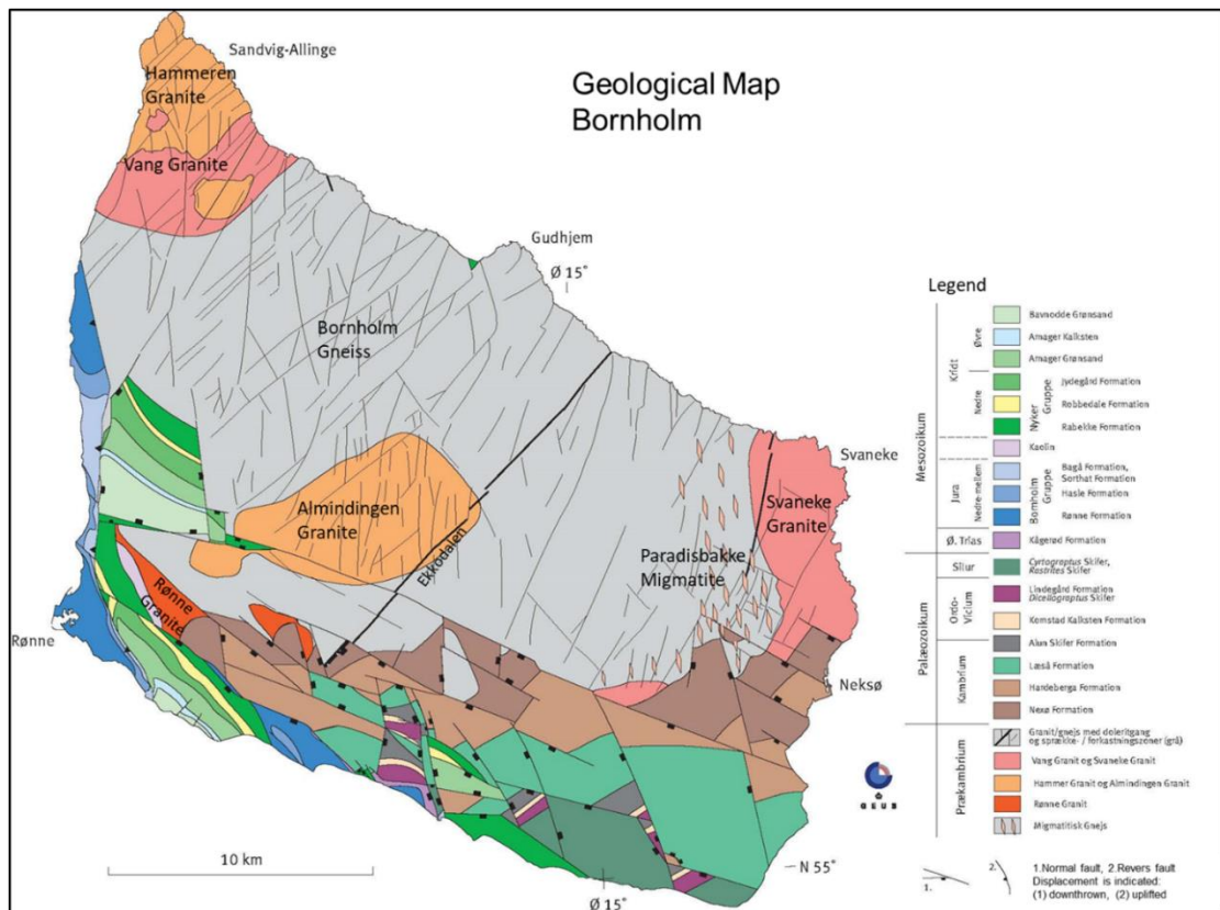
Figure 7. Geological map of Bornholm
