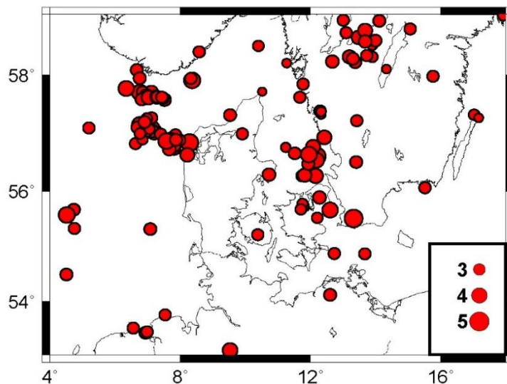
Figure 43. Map showing the location of the largest earthquakes registered in Denmark with magnitudes from 3 to just below 5 on the Richter scale.
