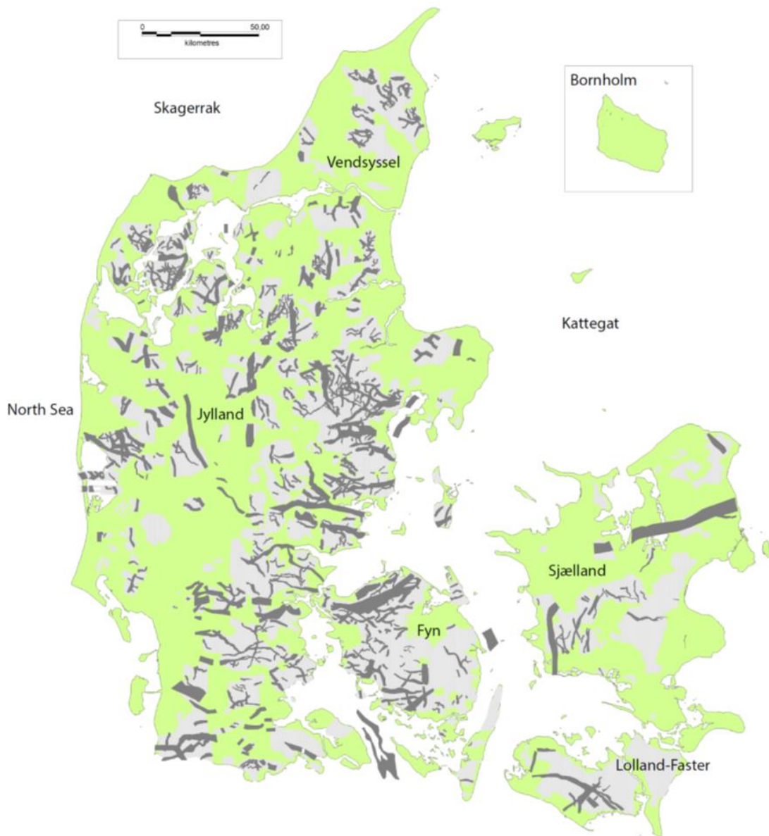
Figure 30. Mapped buried valleys in Denmark shown with dark grey polygons. The light grey areas show the areas with data from Transient Electromagnetic surveys (TEM). Modified from Sandersen & Jørgensen (2017).
