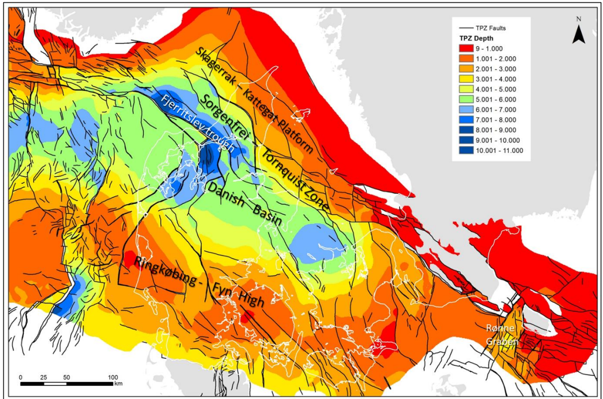
Figure 2. Depth structure map at Top Pre-Zechstein illustrating the setting of the Danish Basin depocenter bounded by the Sorgenfrei-Tornquist Zone to the north and the Ringkøbing – Fyn High to the south. The Rønne Graben is situated in the southeasternmost part of the Sorgenfrei-Tornquist Zone.
