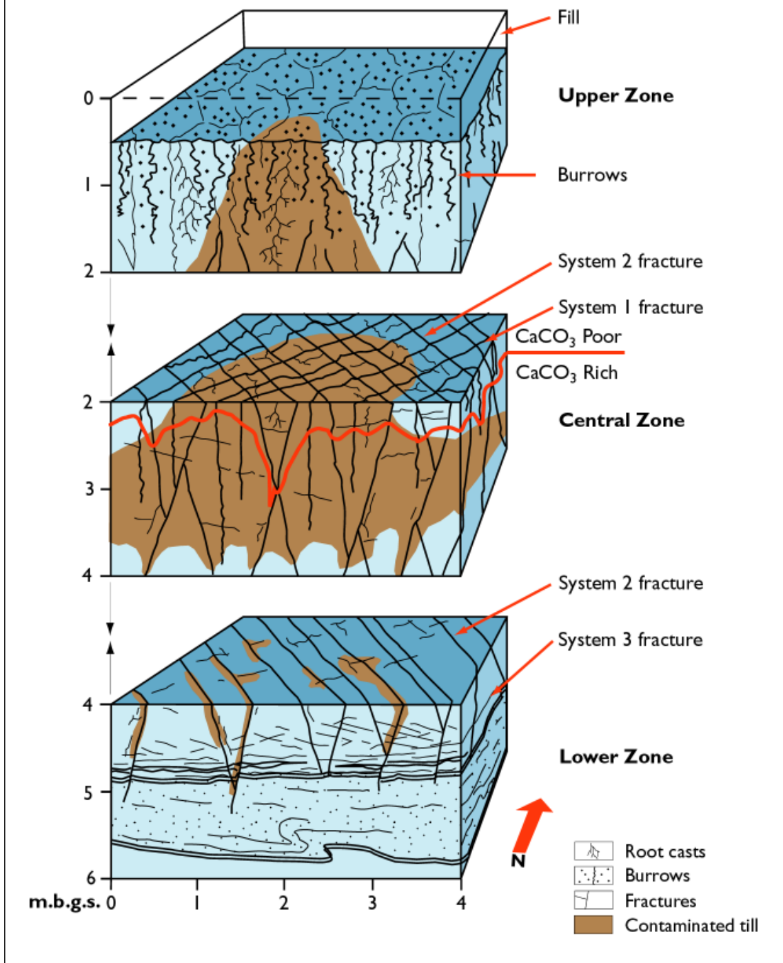
Figure 36. Model of the macropore/fracture systems in a clayey till, Flakkebjerg. (From Klint & Gravesen, 1999).
