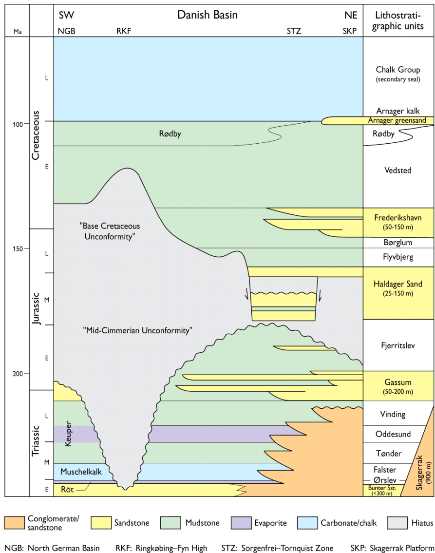
Figure 11. Stratigraphic scheme of the Mesozoic deposits in the Danish and North German Basins (From Nielsen, 2003).
