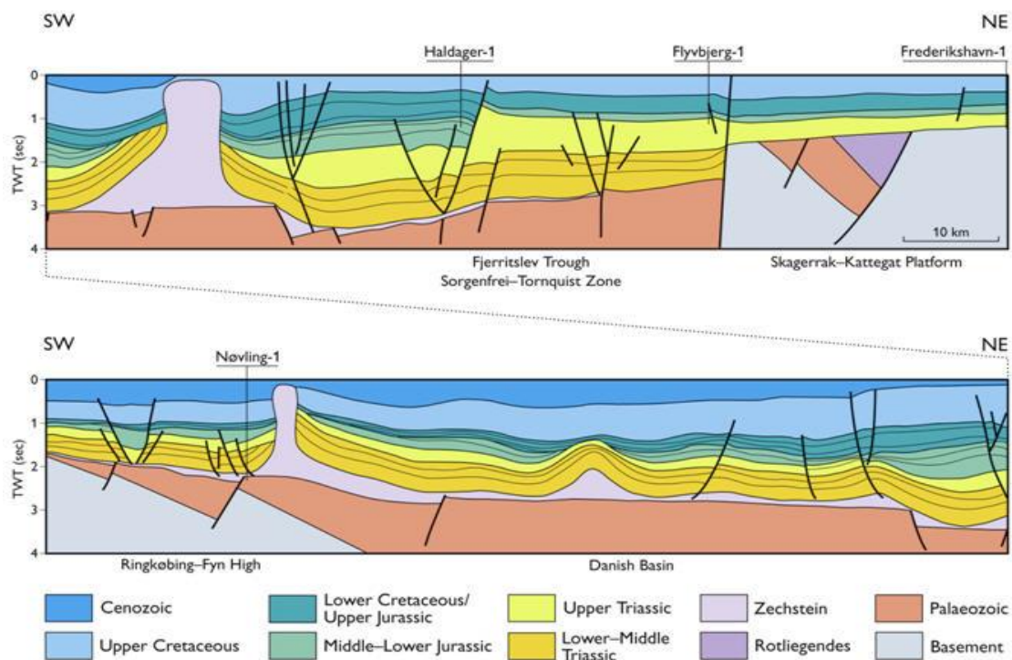
Figure 6. Geological cross section from the Frederikshavn-1 Well, Northern Jylland (NE) to the Nøvling-1 Well, central Jylland (SW) (for location see Figure 5). The section displays about 8 kilometres of section and crosses the Skagerrak- Kattegat Platform, the Sorgenfrei-Tornquist Zone, the Danish Basin and The Ringkøbing-Fyn High (from Nielsen, 2003).
