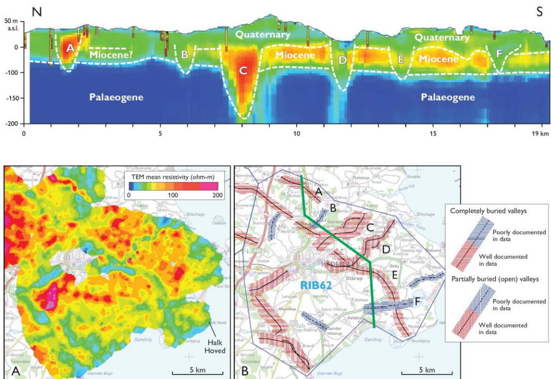
Figure 31. Example of mapping buried valleys using geophysical TEM data. A) Map of recorded resistivity. B) Interpretation of the buried valley systems from combined geophysical data and borings. The status and documentation are noted to the right. The green line in the map indicate the position of the cross section shown in the upper part of the figure. The cross-section in the upper part of the figure illustrates the buried valleys have eroded into geological formations from the Miocene and Palaeogene (from Sandersen & Jørgensen, 2017).
