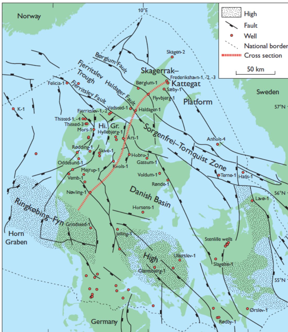
Figure 5. Map of the geological structural framework of Denmark including the Sorgenfrei-Tornquist Zone, the Ringkøbing-Fyn High, the Skagerrak-Kattegat Platform, the Danish and German Basins and several associated faults. Deep wells are located with red dots. For Bornholm, see the map in Figure 7 (from Nielsen, 2003).
