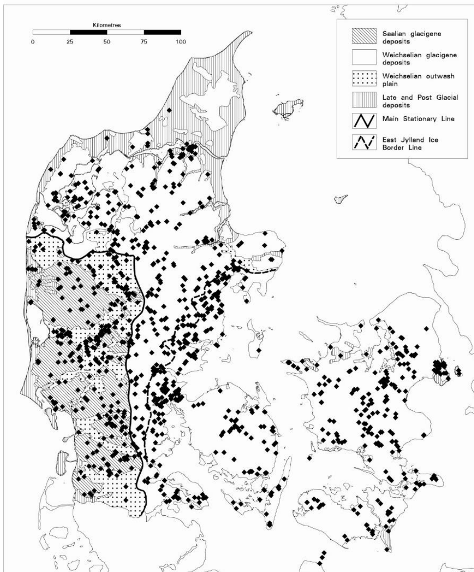
Figure 29. Map showing the location of boreholes with borehole logs where dislocated pre-Quaternary sediments are recorded above or within the Quaternary deposits (From Jakobsen, 1996).
