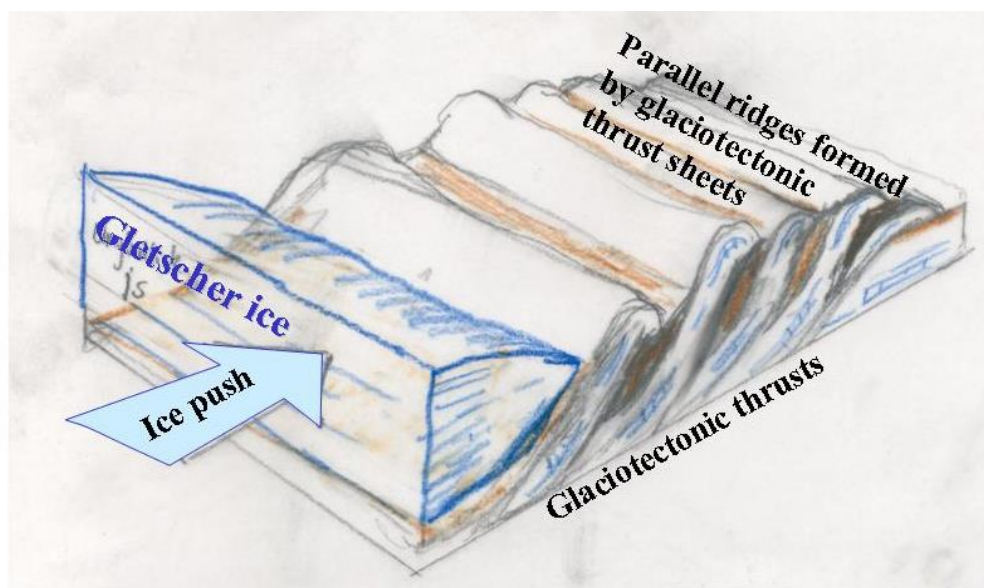
Figure 28. Conceptual diagram illustrating a glaciotectonic complex. The glaciotectonic thrust faulting creates a landscape with parallel ridges perpendicular to the direction of the ice push. The thickness of the thrust sheets is 50–100 m, and the crests are elevated up to 100 meters above the original depositional position of the layers. Along strike, the crests may extend up to 10 kilometres.
