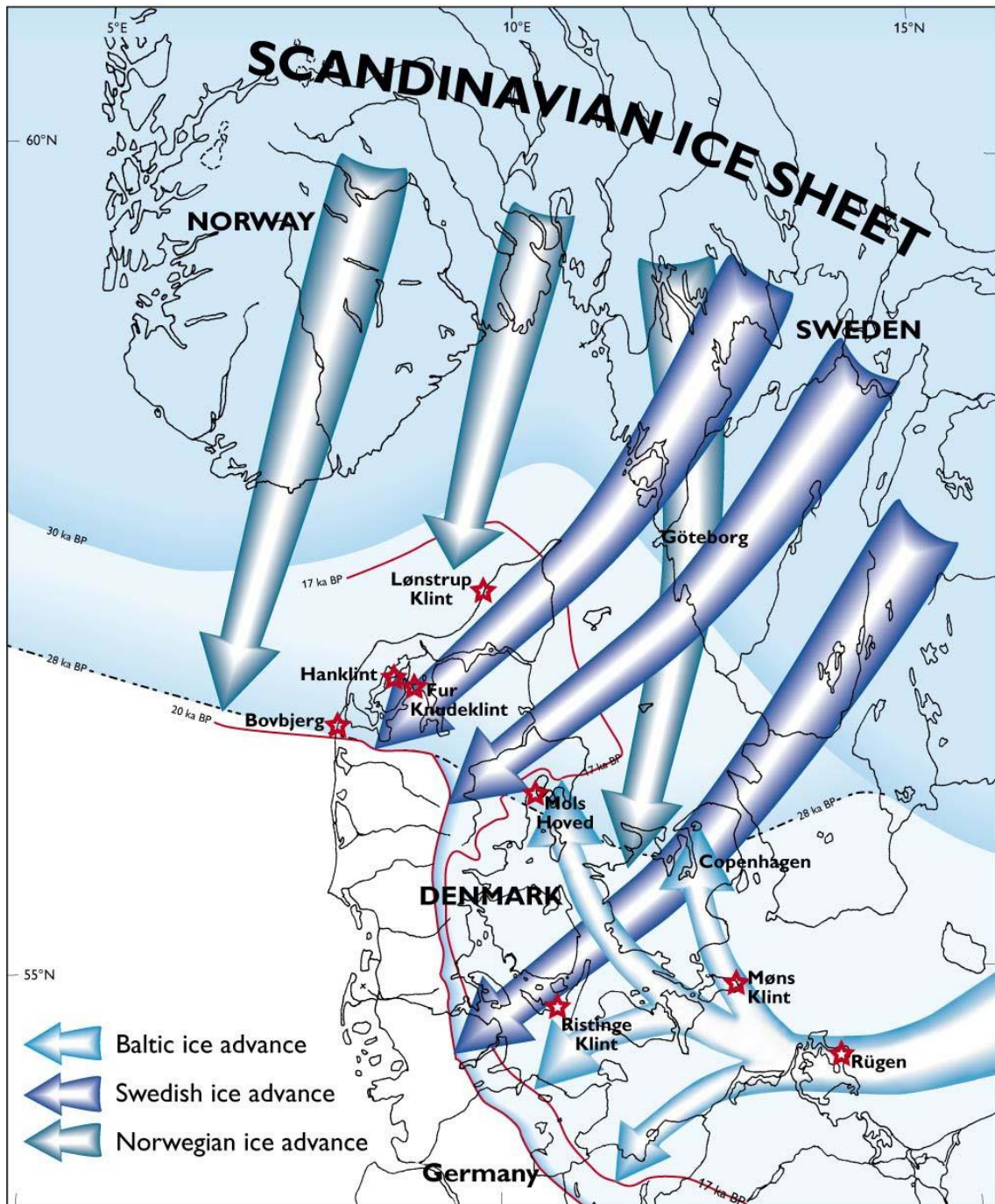
Figure 25. The glacier advances during the Weichselian with three main courses from north, northeast, and southeast. Red asterisks mark larger glaciotectonic complexes in Denmark and on Rügen, N Germany (From Pedersen, 2005).
