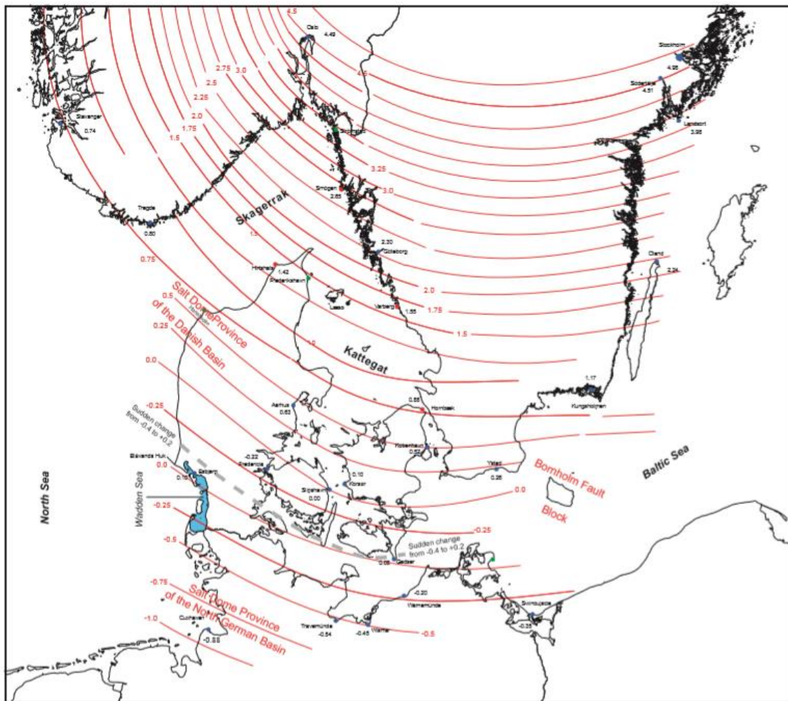
Figure 32. Map showing the present-time isostatic uplift rates (red lines) of the Danish and surrounding areas in mm/year. The dashed, grey line shows the boundary between the northern areas that are currently being uplifted and southernmost areas where subsidence is ongoing (From Hansen et al. 2012).
