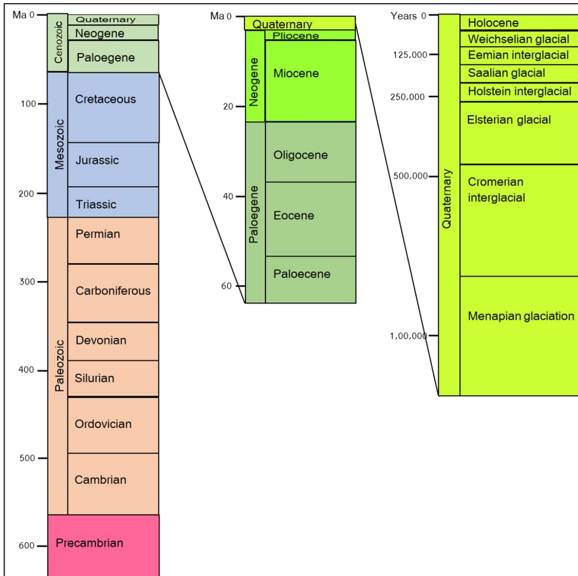
Figure 4. Geological time periods overview referred in this report
