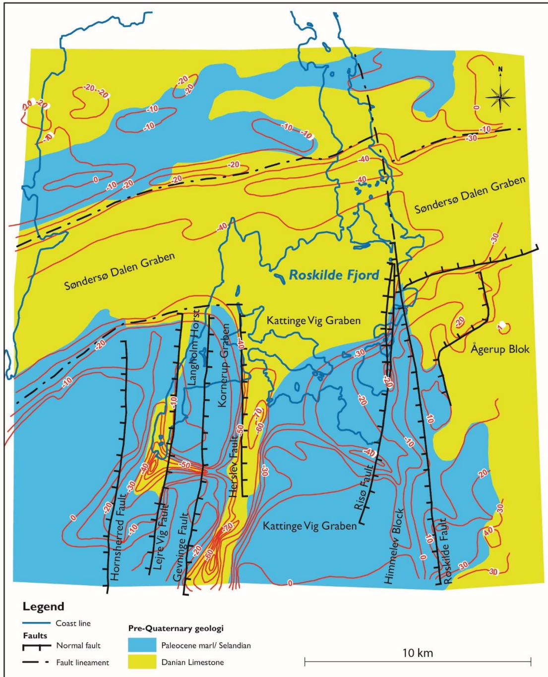
Figure 9. Map of the pre-Quaternary surface in the Roskilde Fjord area showing that several small faults and graben systems are recognized. The contour lines outline the topography of the pre-Quaternary surface (meters below mean sea level). (From Gravesen & Pedersen, 2005).
