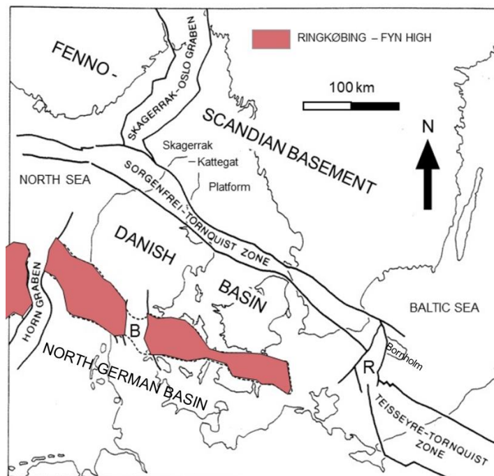
Figure 2. The structural elements of the Danish subsurface, which is governed by the position of the Ringkøbing–Fyn High. B is the location of the Brände Through, and R indicates the Rønne Graben, which forms the western boundary of the basement horst comprising the main part of the island Bornholm.
