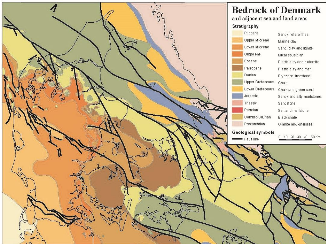
Figure 22. Map of the geological units outcropping at the pre-Quaternary surface. A general trend is that younger units appear towards the WSW, ranging from Precambrian basement in Sweden to the Miocene/Pliocene deposits in SW Jylland. Modified after Håkansson & Pedersen, 1992.
