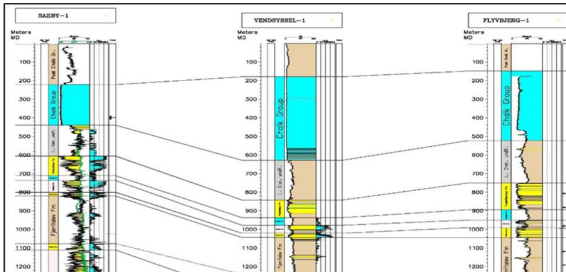
Figure 18. An example of well log correlation based on petrophysical logs and core descriptions: Saeby-1, Vendsyssel-1, and Flyvbjerg-1. The blue interval in the upper part is Upper Cretaceous, the underlying interval of varied colours is Lower Cretaceous (For location see Figure 3, from Nielsen, 2003).
