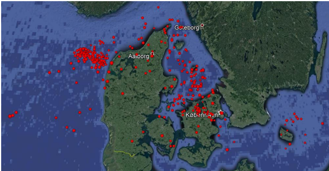
Figure 42: Instrumentally recorded seismicity in Denmark for the period 1930 – 2018. Epicenters (red dots) are from GEUS earthquake database, and all epicenters are determined using data from a minimum of three stations. In addition to earthquakes the map may show data related to explosions which have not yet been screened out (GEUS, 2018).
