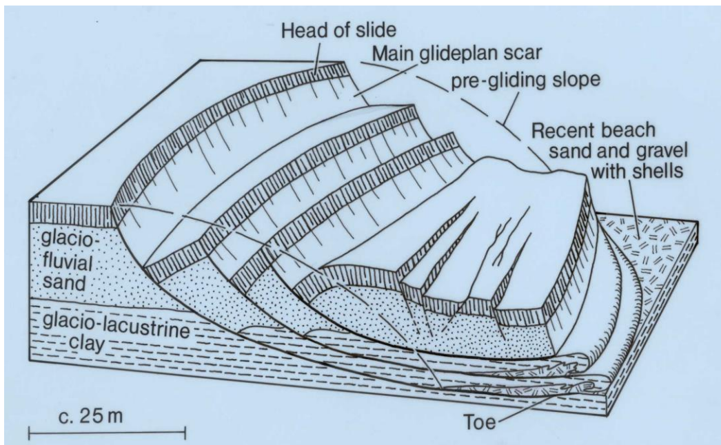
Figure 39. A model of the structural elements of the landslide (after Pedersen 1987).
