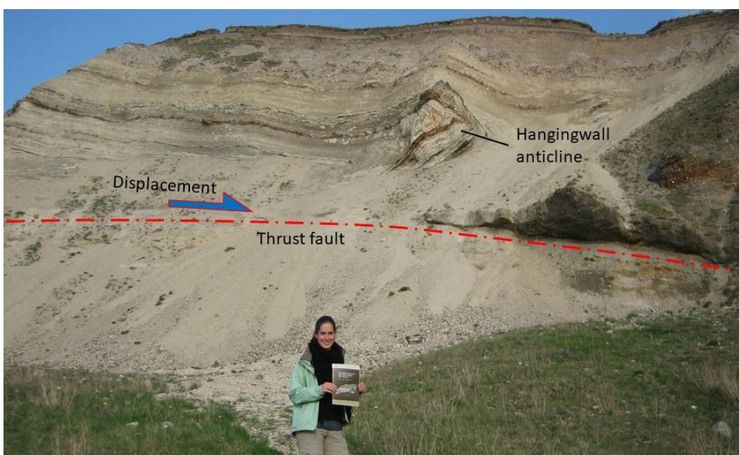
Figure 27. An example of Weichselian glaciotectonic deformation, the Hanklit thrust sheet on northern Mors. This thrust sheet comprises Eocene clayey diatomite with volcanic ash layers, and it was laterally displaced c. 300 meters across Pleistocene outwash deposits.
