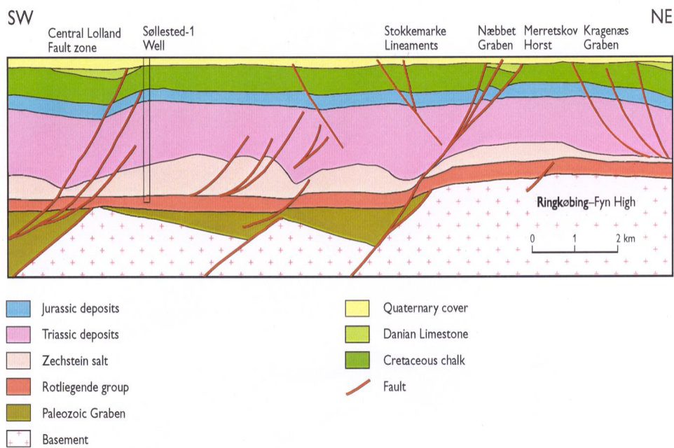
Figure 8. Geological cross section from the northern part of Lolland showing the fault patterns extending from the basement up into the Danian sediments and perhaps also extending into the Quaternary sediments (from Pedersen et al., 2015).
