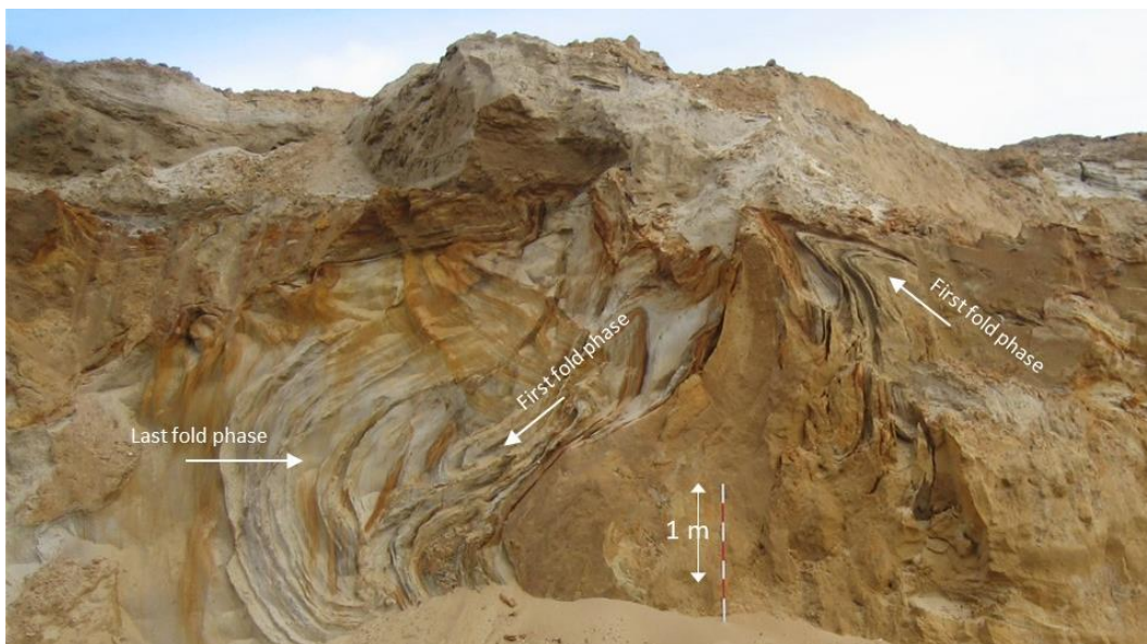
Figure 26. An example of glaciotectonic deformation in the Saalian landscape. Superimposed folding in glaciofluvial sand, Attenager, Ringkøbing.
