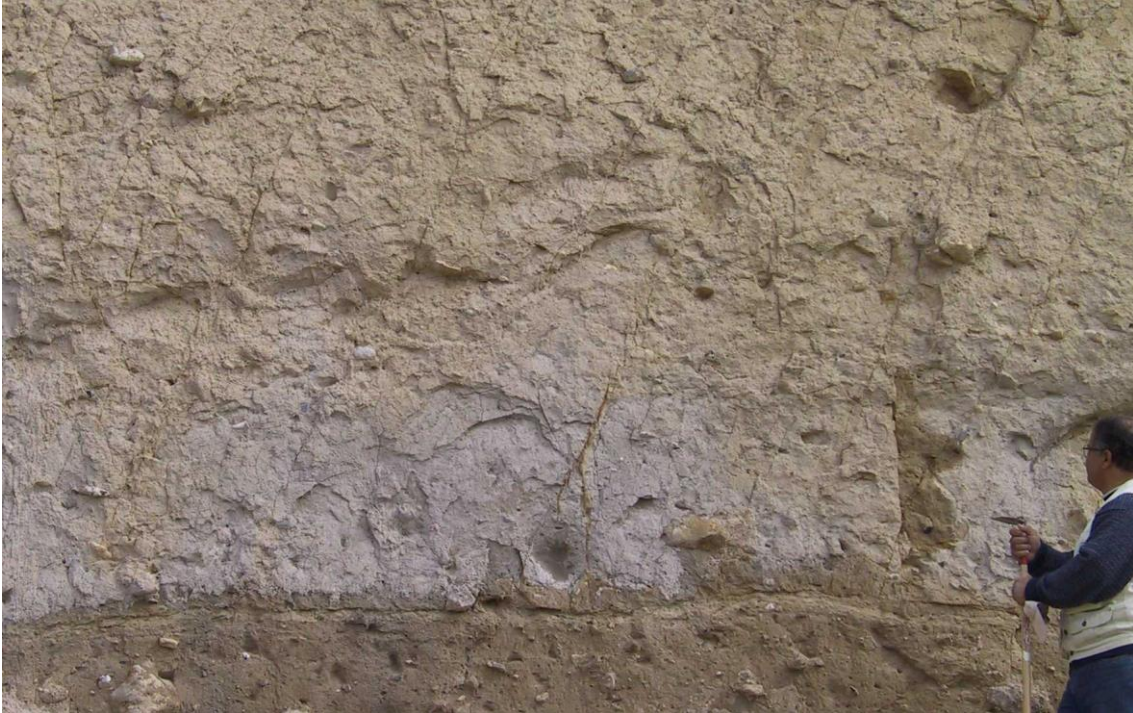
Figure 35. Outcrop of clayey till in a gravel pit, Sjælland. Sets of sub-vertical fractures can be recognized.
