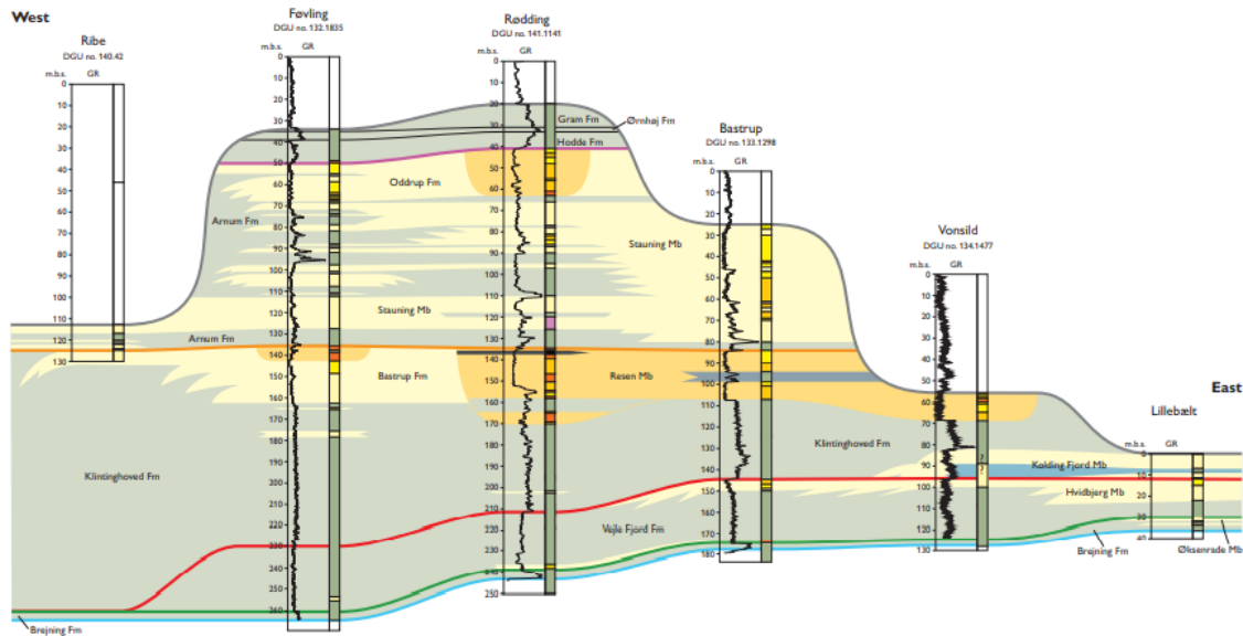
Figure 3.10. Stratigraphic well log correlation showing that the amounts of sand and claystone, respectively, vary significantly both horizontally (from west to the east across southern Jylland) and vertically through the Miocene record (Rasmussen et al., 2010). The yellow and orange colours show the presence of sand and gravel, the greyish colours show mudstone dominated sediments.
