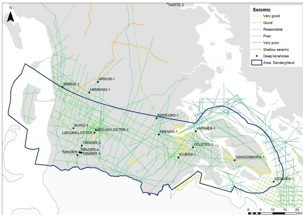
Figure 6.74. Location map showing seismic lines and their quality, and deep boreholes in the Søndersjylland area. In this area, the seismic data coverage is relatively good.
