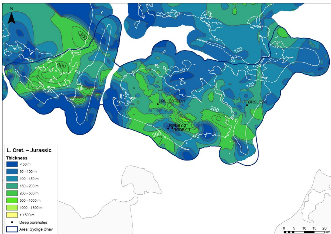
Figure 6.112. Thickness map of the combined Lower Cretaceous and Jurassic successions, Sydligge Øhav area. The thickness varies between 50 and 500 meters over short distances due to the Lower Jurassic successions occurring in fault-bounded half grabens (Figure 4.21).
