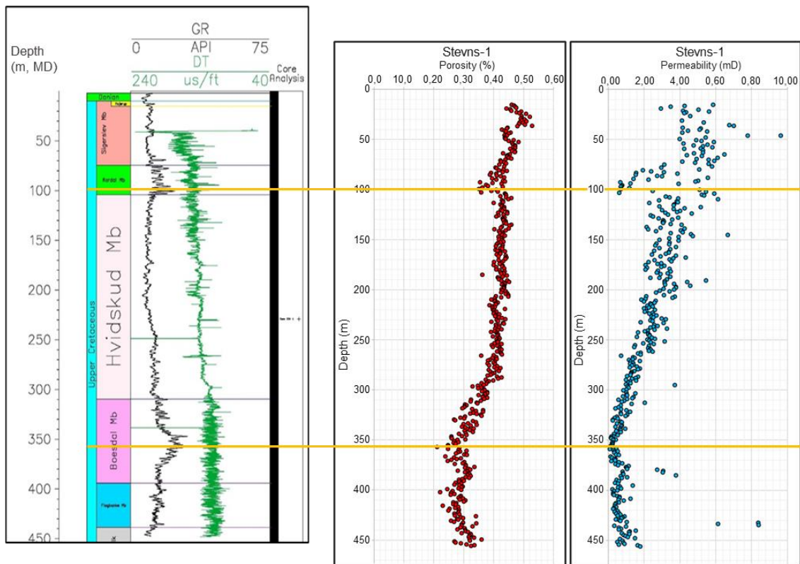
Figure 3.7. The figure to the left shows two combined petrophysical logs (gamma log GR, and sonic log representing 1/sound velocity, DT) from the Stevns-1 borehole (Kristensen et al. 2016). A high clay content is interpreted where GR-readings are high, at the depths marked with yellow lines. The high clay content coincides with low porosities and permeabilities as plotted in the diagrams to the right (Mortensen et al., 1998). Generally, such a correlation between low porosity and permeability, and high clay content is expected as clay rich sediments show a high degree of compaction due to the minerals' plate structure. The increased amounts of clay in the Stevns-1 well occur in the Boesdal Member and Rørdal Member, which are known from other areas to comprise significant amounts of clay (see also Report no. 3).
